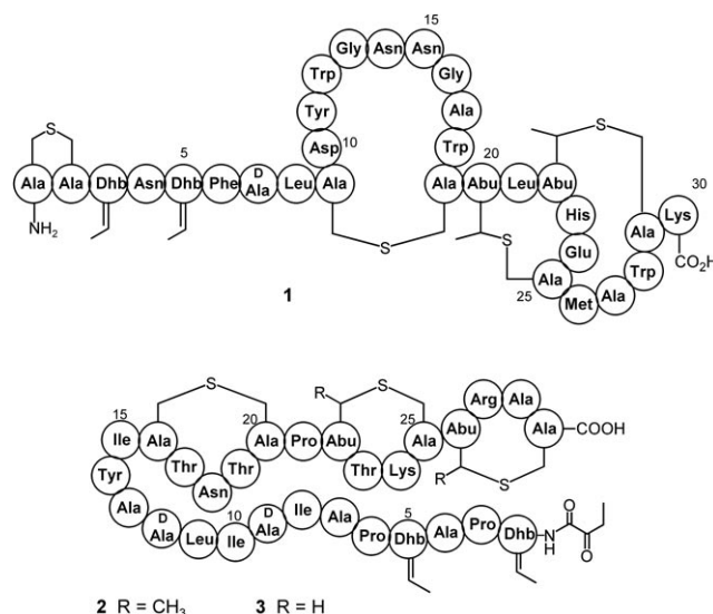
Figure 1. Lactacin 3147 components A1 ( 1 ) and A2 ( 2 ). The bis(desmethyl) lanthionine analogue ( R = H ) of lactacin A2 is Lan-A2 ( 3 ). It is proposed that the \alpha -carbon atoms of residues 26, 22, and 16 in 2 , and alanine residues 9 and 12 have the D configuration. [5]
